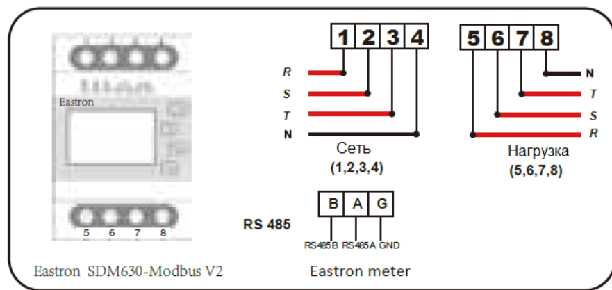
Parallel_A Parallel_B Meter-485 port
